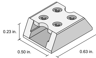
DI-TB8-CONN-TTT (Tape-to-Tape)
