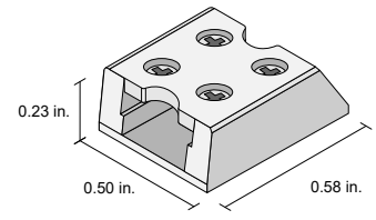
DI-TB8-CONN-TTW (Tape-to-Wire)
